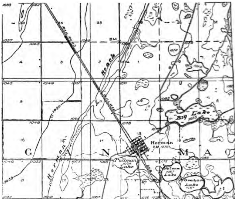
FIG. 357. — Portion of the Herman quadrangle of Minnesota, showing the position of the Herman beach on the shore of the former Lake Agassiz. The lake basin is to the left, and the pitted morainal deposits appear to the right (U. S. G. S.).
